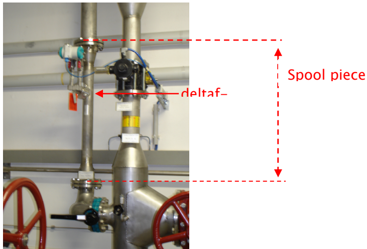
Figure 5 Spool piece (weld-in type) with integrated deltaflow and reduction in
